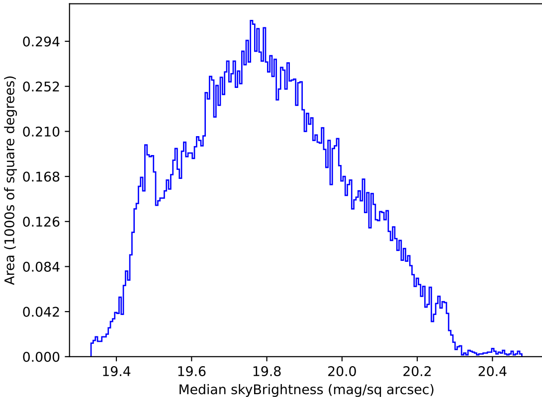
noroll_v3.4_10yrs All sky all bands: Median skyBrightness
