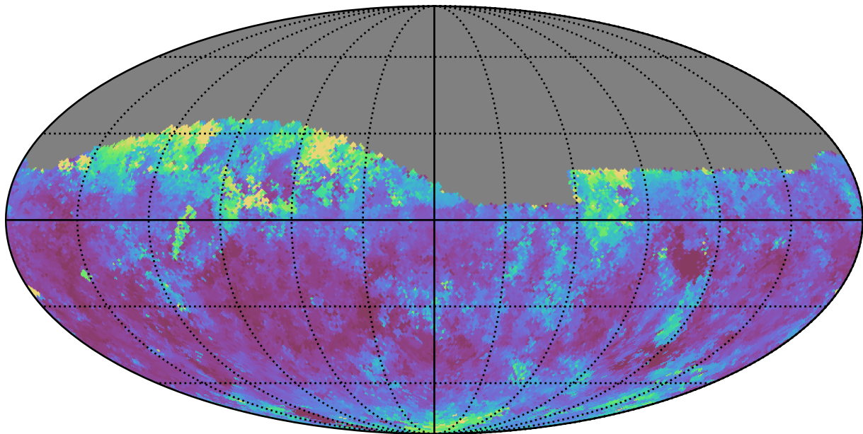
noroll_v3.4_10yrs Yr 1 z band: Median seeingGeom
