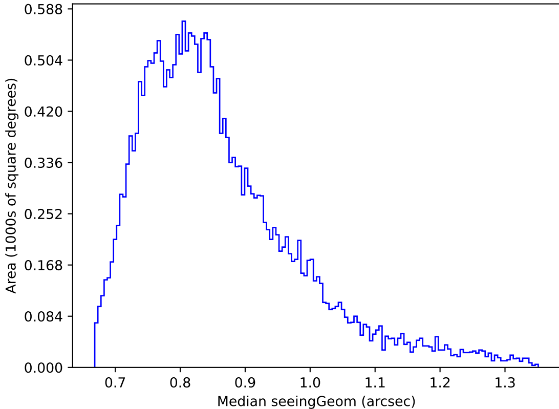
noroll_v3.4_10yrs Yr 1 z band: Median seeingGeom
