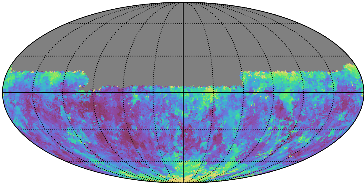
noroll_v3.4_10yrs Yr 1 y band: Median seeingGeom
