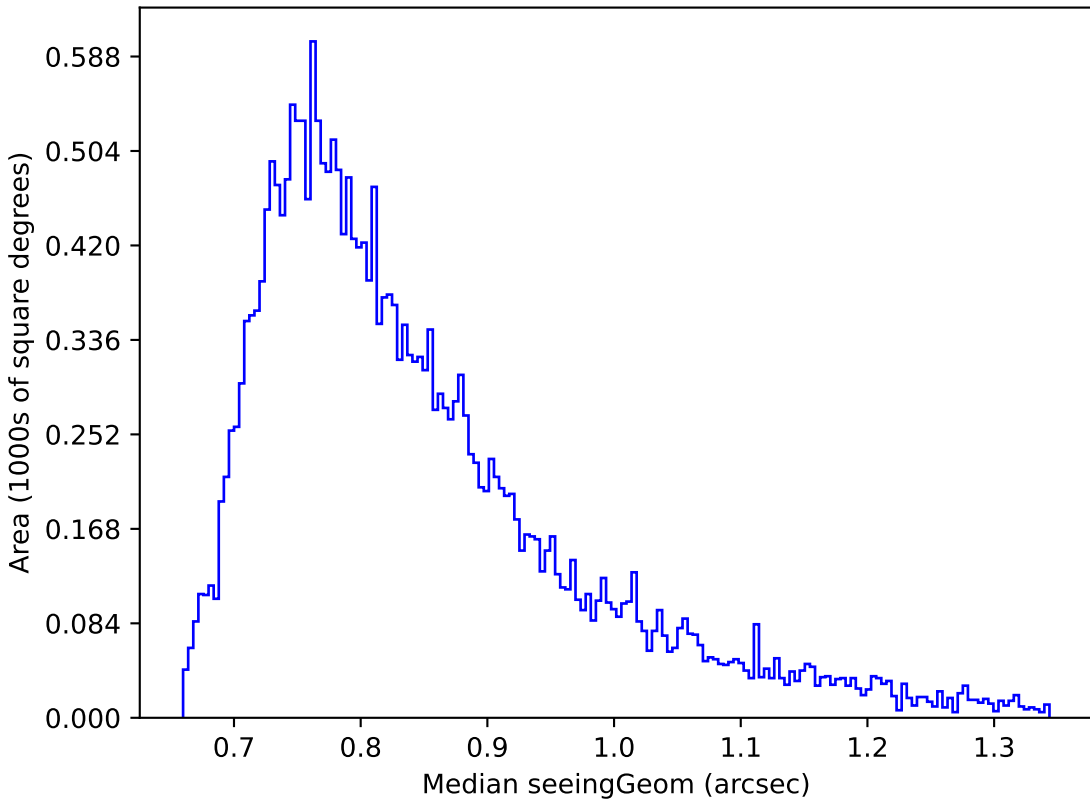
noroll_v3.4_10yrs Yr 1 r band: Median seeingGeom
