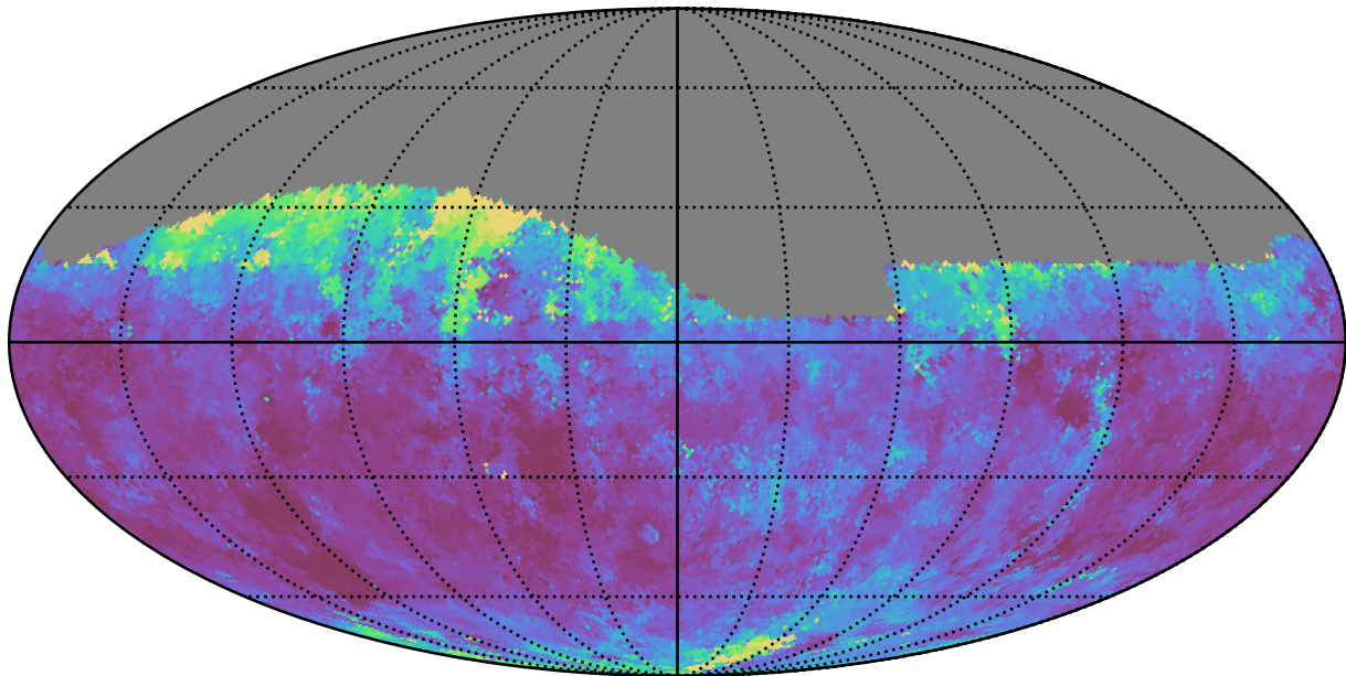
noroll_v3.4_10yrs Yr 1 i band: Median seeingGeom
