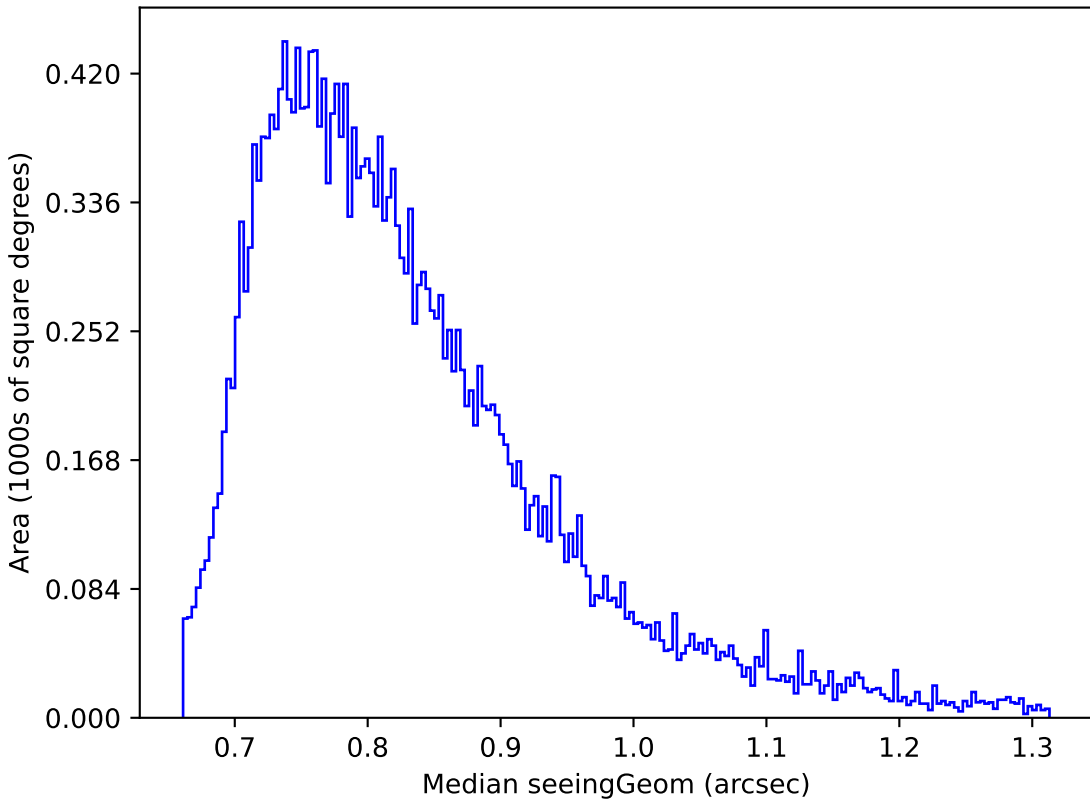
noroll_v3.4_10yrs Yr 1 i band: Median seeingGeom
