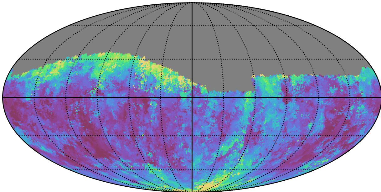
noroll_v3.4_10yrs Yr 1 g band: Median seeingGeom
