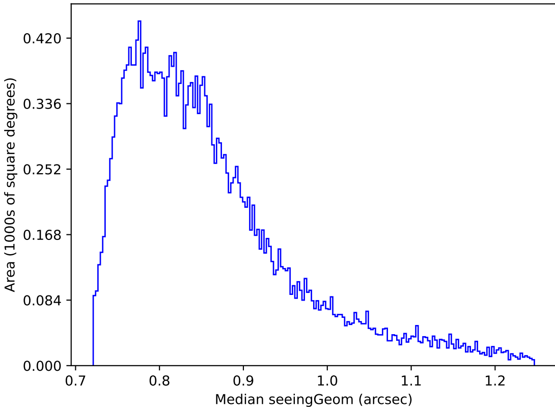
noroll_v3.4_10yrs Yr 1 all bands: Median seeingGeom
