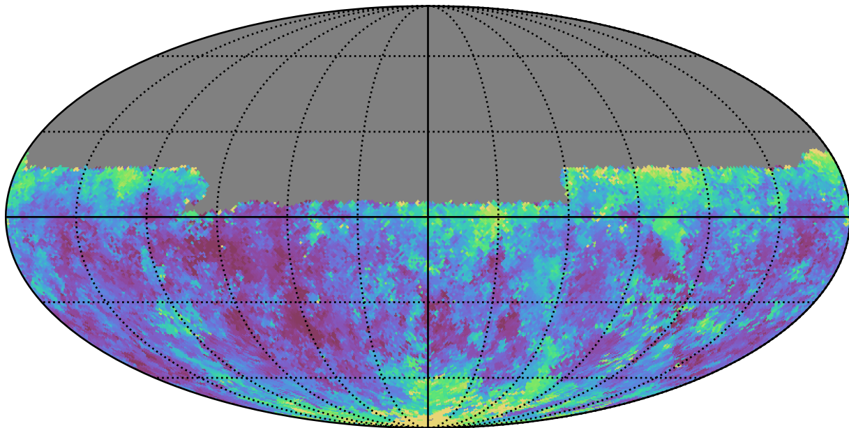
noroll_v3.4_10yrs Yr 1 y band: Median seeingEff
