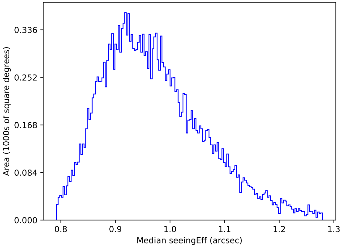
noroll_v3.4_10yrs Yr 1 y band: Median seeingEff
