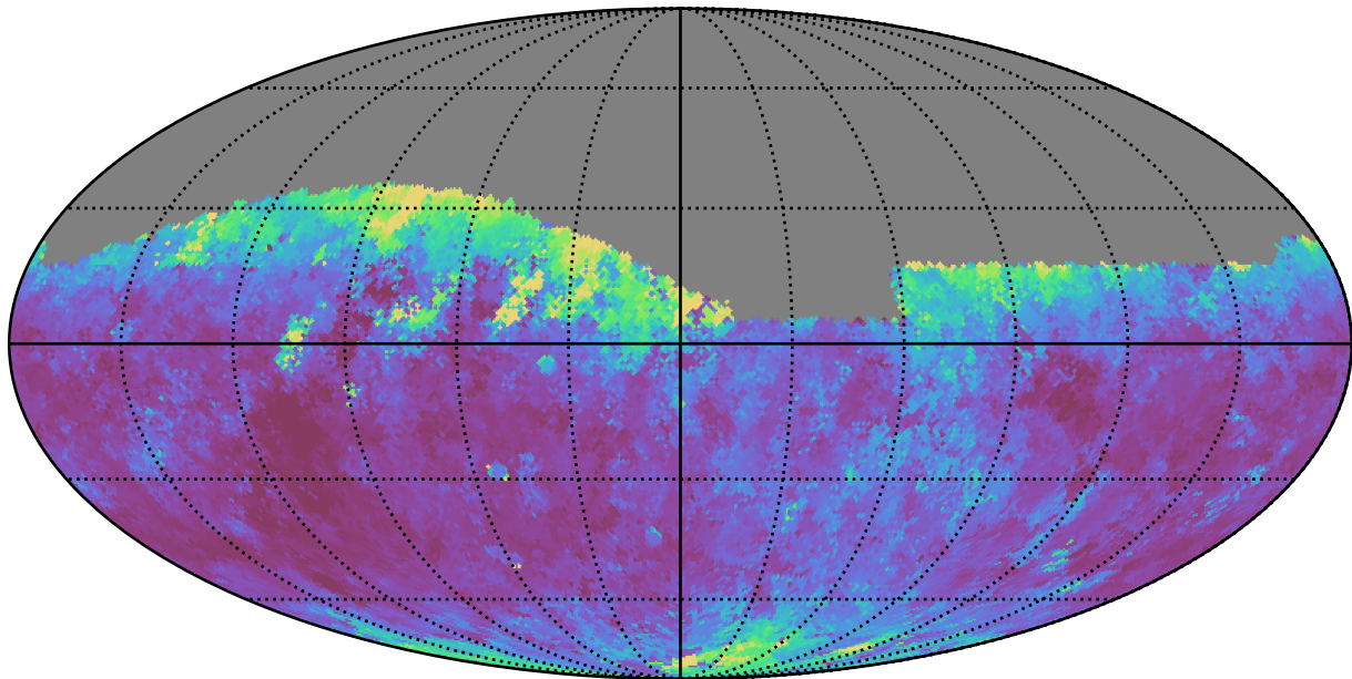
noroll_v3.4_10yrs Yr 1 r band: Median seeingEff
