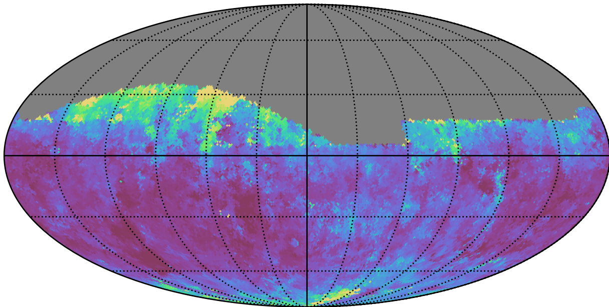
noroll_v3.4_10yrs Yr 1 i band: Median seeingEff
