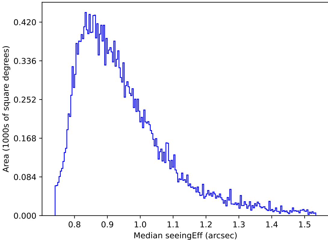
noroll_v3.4_10yrs Yr 1 i band: Median seeingEff
