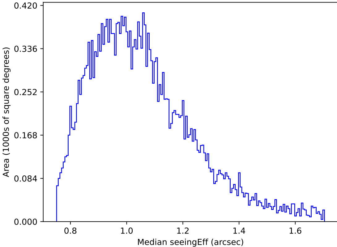
noroll_v3.4_10yrs Yr 1 g band: Median seeingEff
