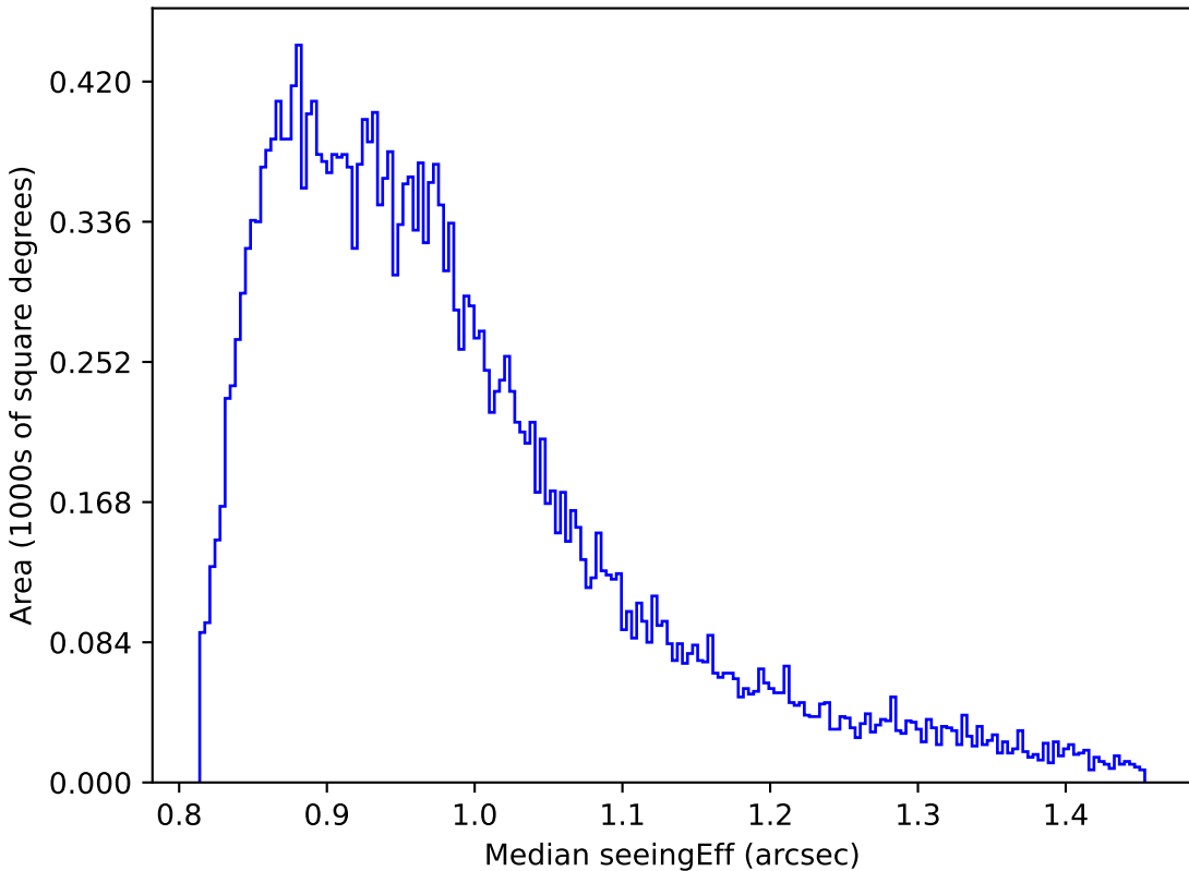
noroll_v3.4_10yrs Yr 1 all bands: Median seeingEff
