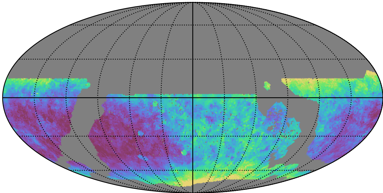
noroll_v3.4_10yrs WFD z band: Median seeingEff
