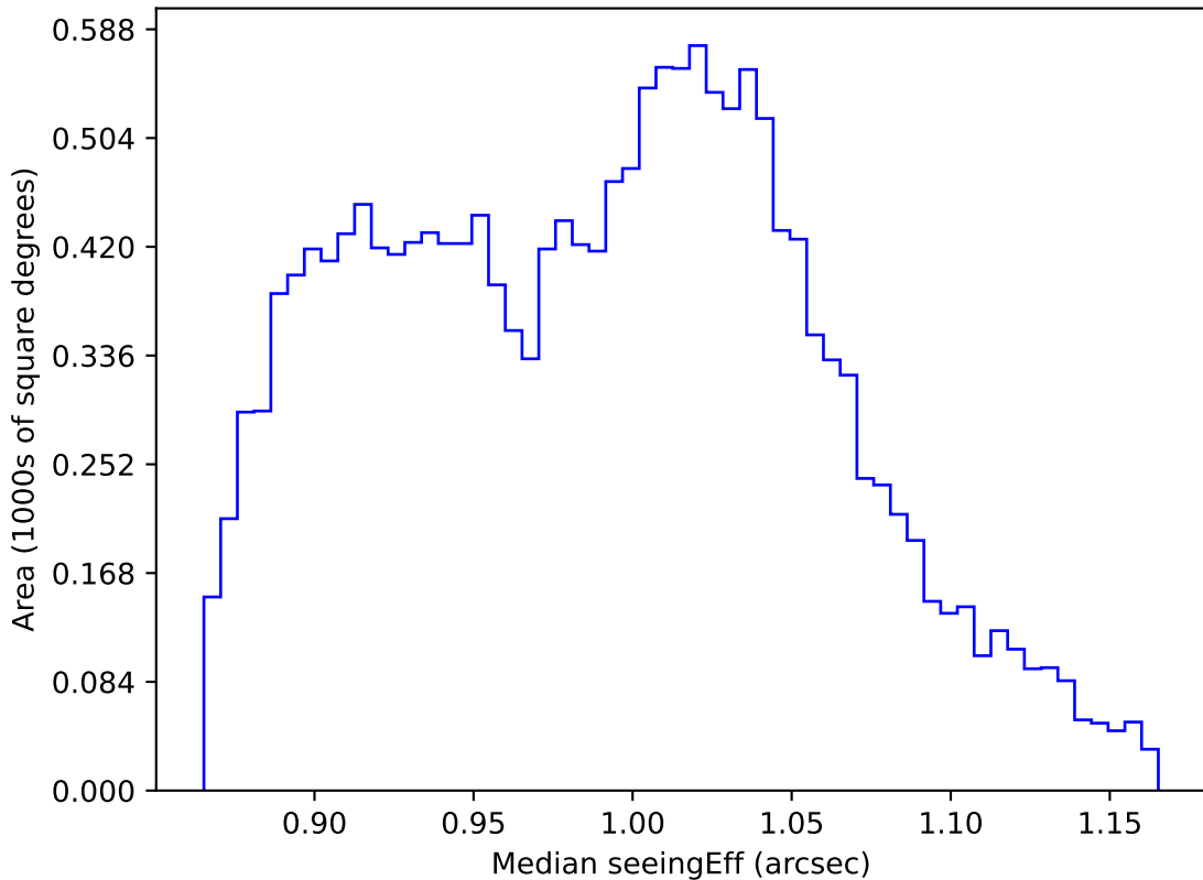
noroll_v3.4_10yrs WFD z band: Median seeingEff
