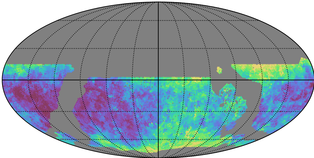
noroll_v3.4_10yrs WFD u band: Median seeingEff
