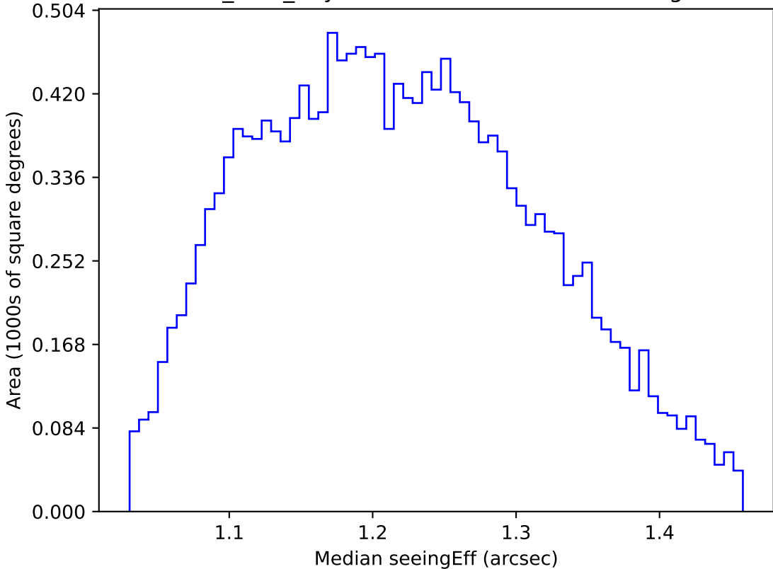
noroll_v3.4_10yrs WFD u band: Median seeingEff
