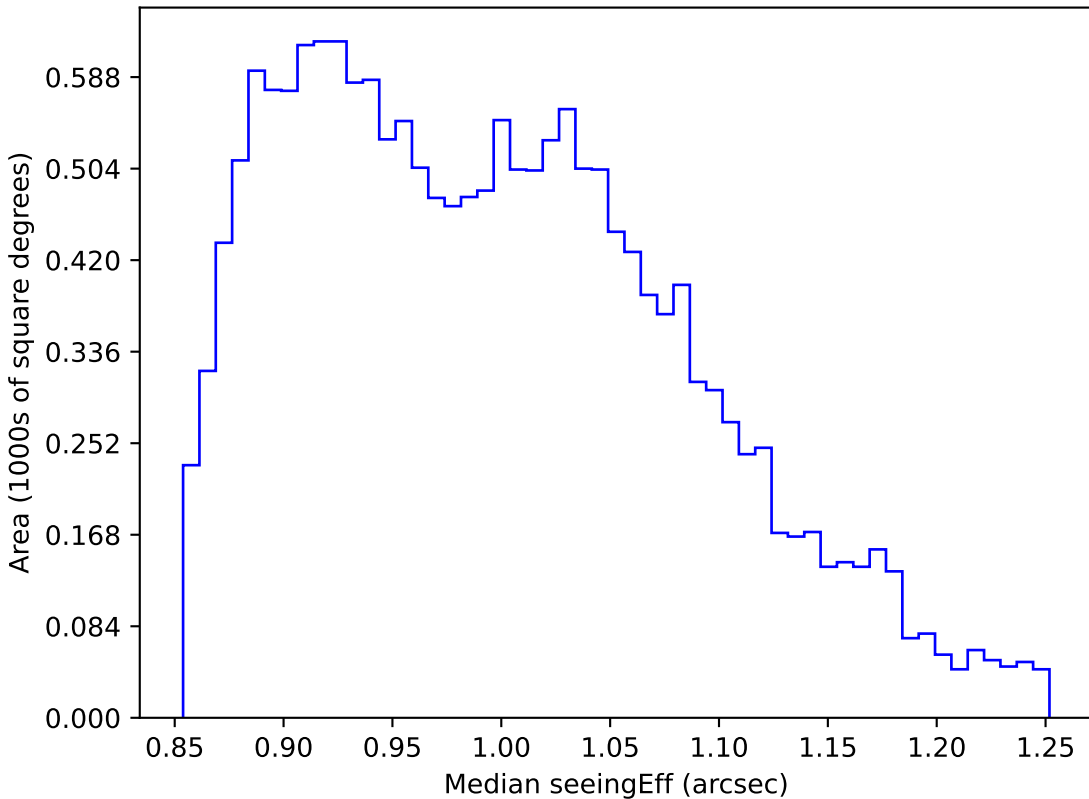
noroll_v3.4_10yrs WFD r band: Median seeingEff
