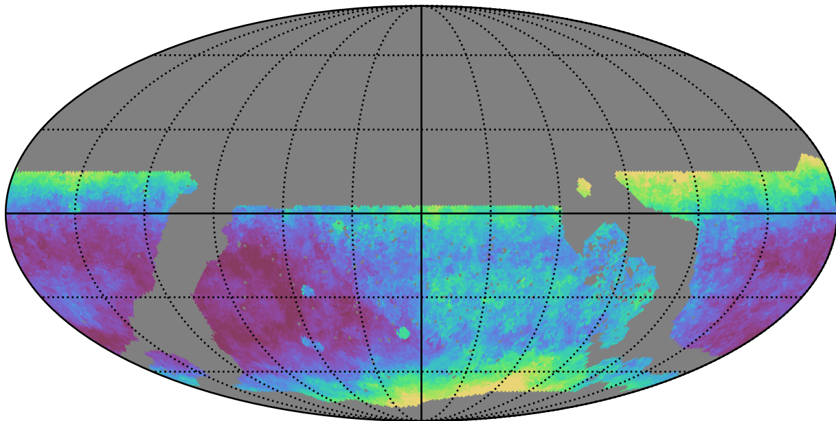
noroll_v3.4_10yrs WFD i band: Median seeingEff
