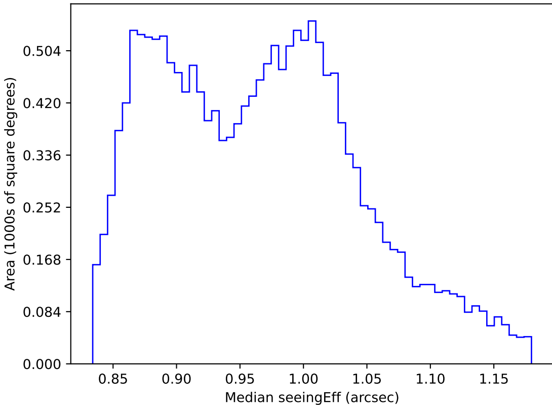
noroll_v3.4_10yrs WFD i band: Median seeingEff
