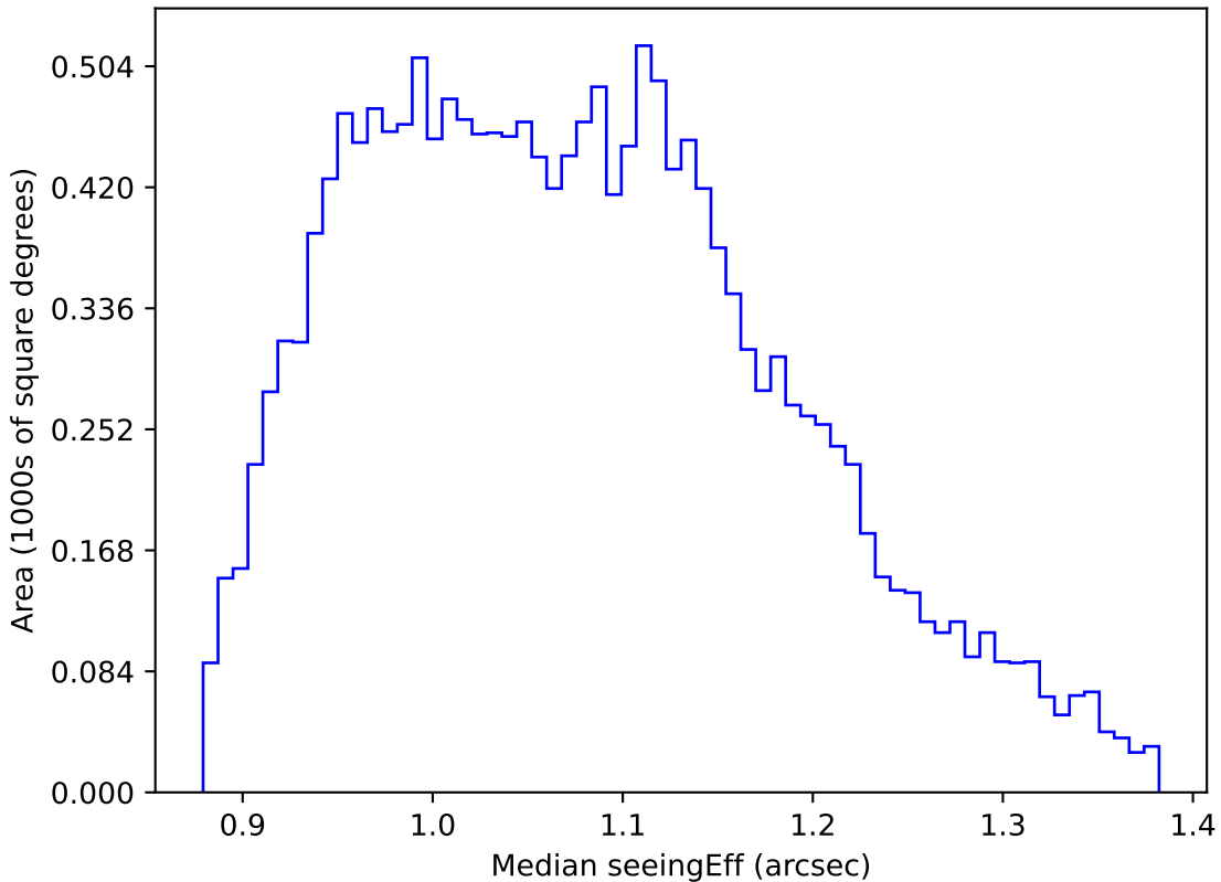
noroll_v3.4_10yrs WFD g band: Median seeingEff
