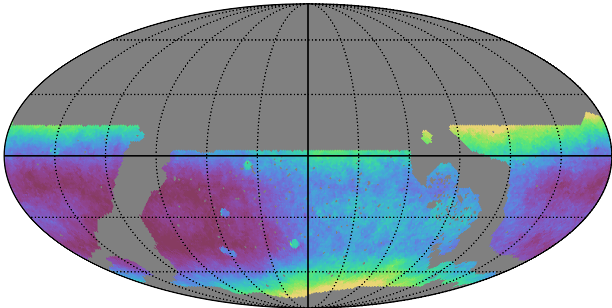
noroll_v3.4_10yrs WFD all bands: Median seeingEff
