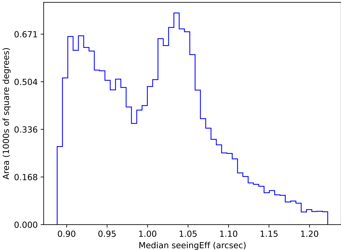
noroll_v3.4_10yrs WFD all bands: Median seeingEff
