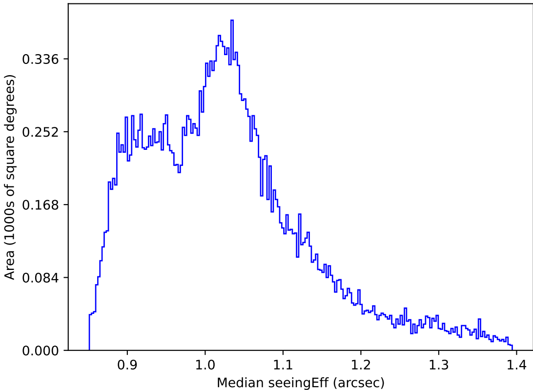
noroll_v3.4_10yrs All sky z band: Median seeingEff
