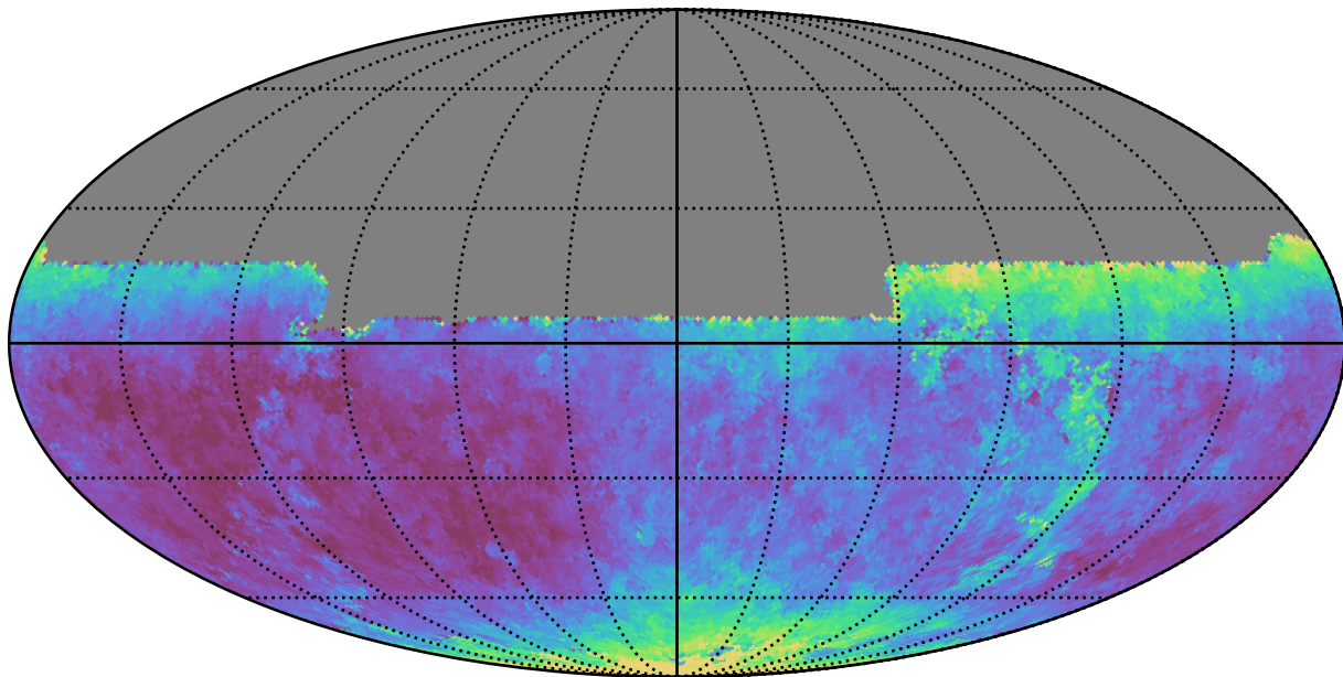
noroll_v3.4_10yrs All sky y band: Median seeingEff
