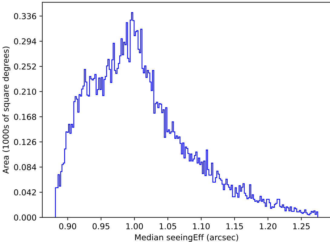
noroll_v3.4_10yrs All sky y band: Median seeingEff
