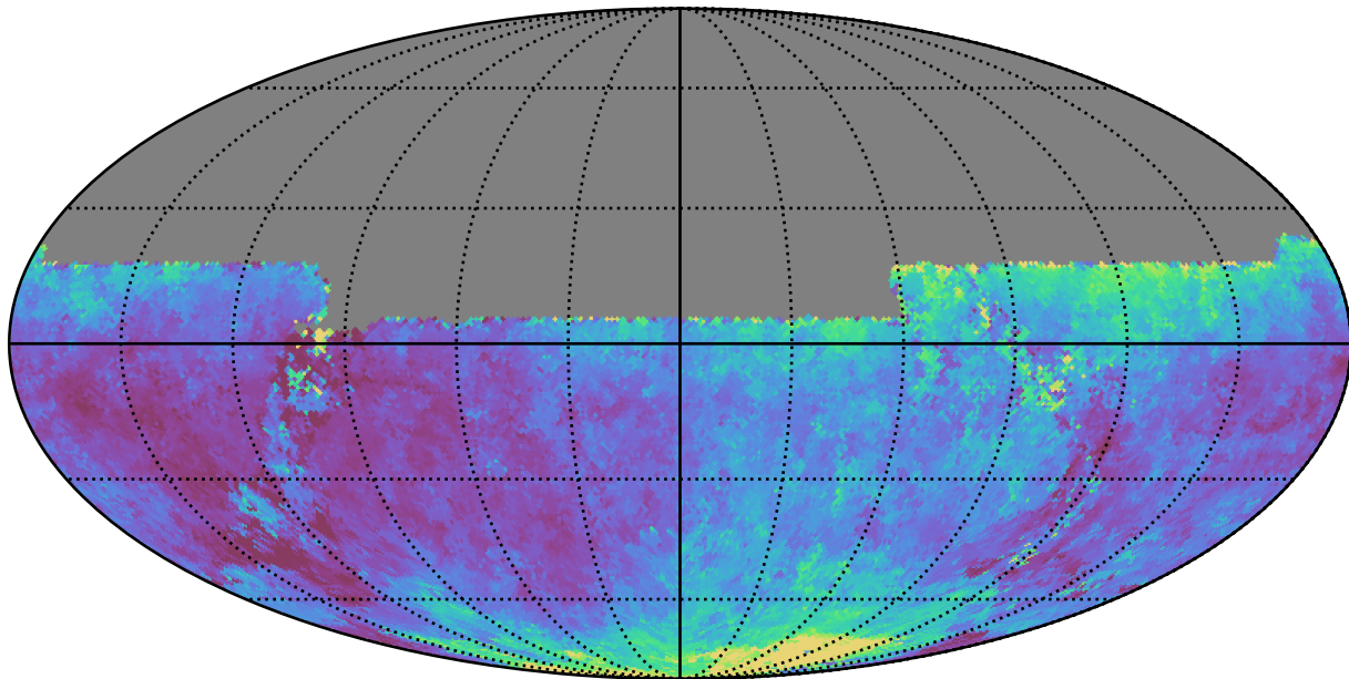
noroll_v3.4_10yrs All sky u band: Median seeingEff
