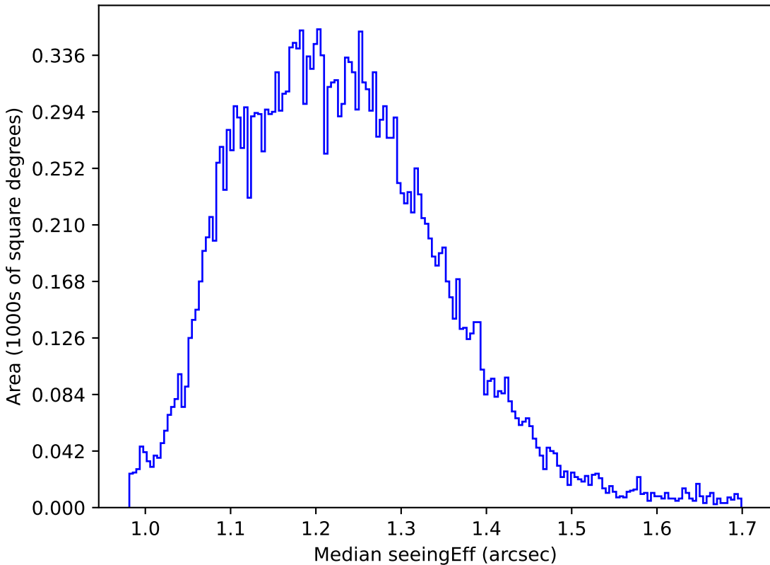
noroll_v3.4_10yrs All sky u band: Median seeingEff
