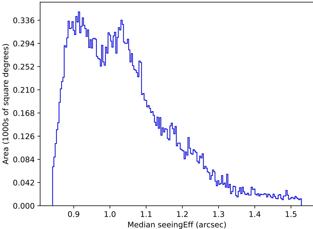
noroll_v3.4_10yrs All sky r band: Median seeingEff
