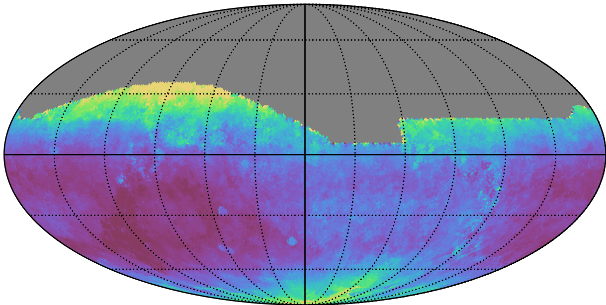
noroll_v3.4_10yrs All sky i band: Median seeingEff
