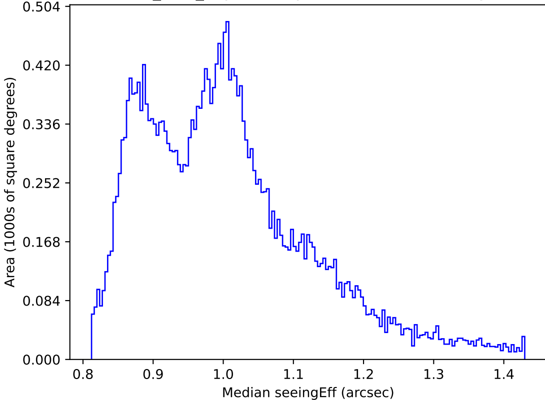
noroll_v3.4_10yrs All sky i band: Median seeingEff
