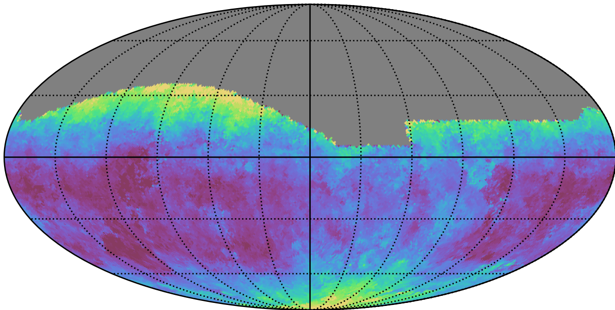
noroll_v3.4_10yrs All sky g band: Median seeingEff
