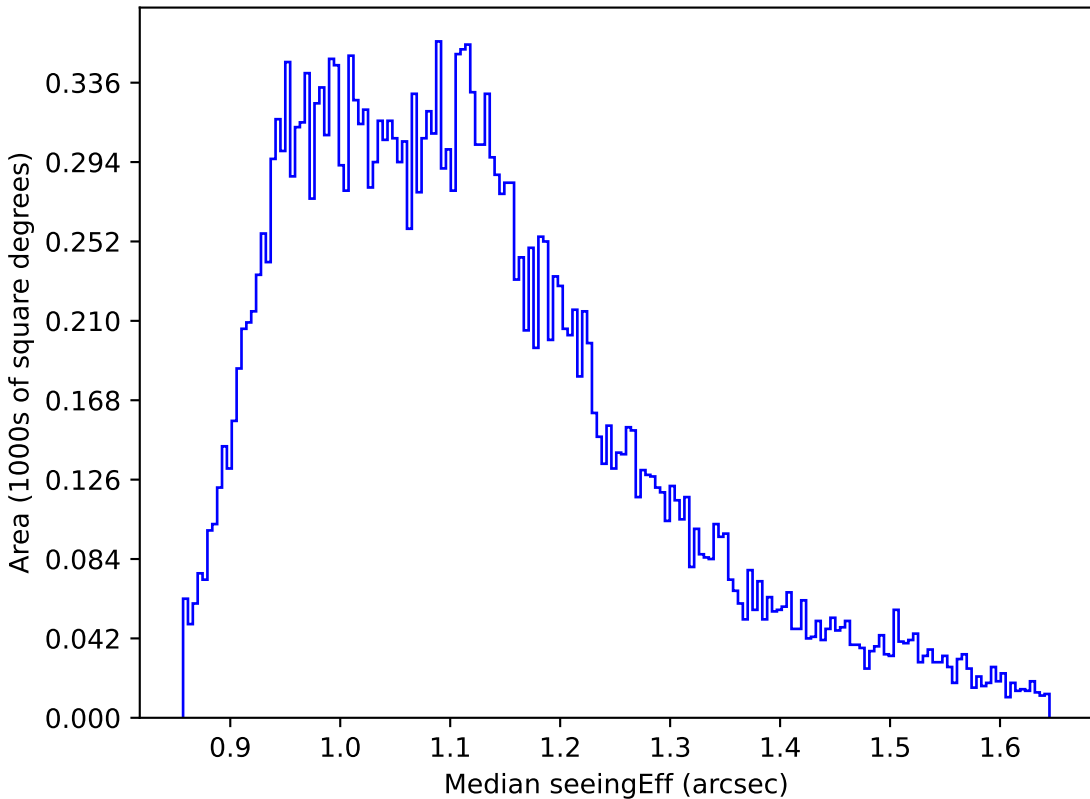
noroll_v3.4_10yrs All sky g band: Median seeingEff
