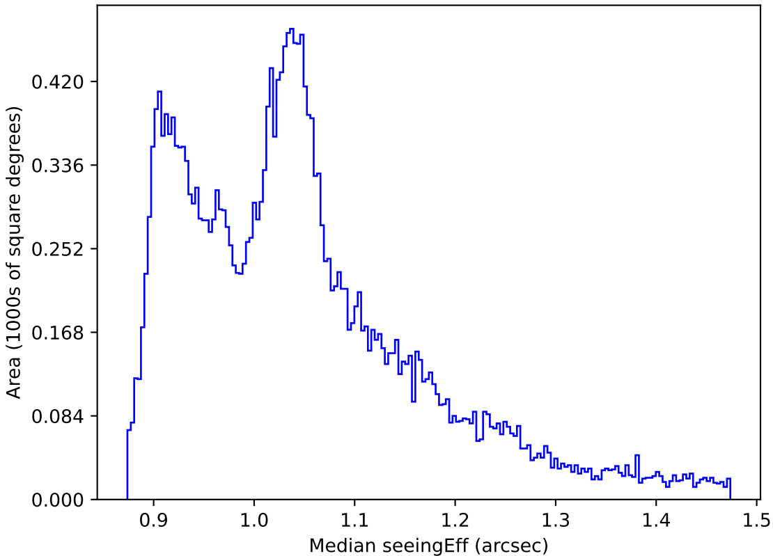
noroll_v3.4_10yrs All sky all bands: Median seeingEff
