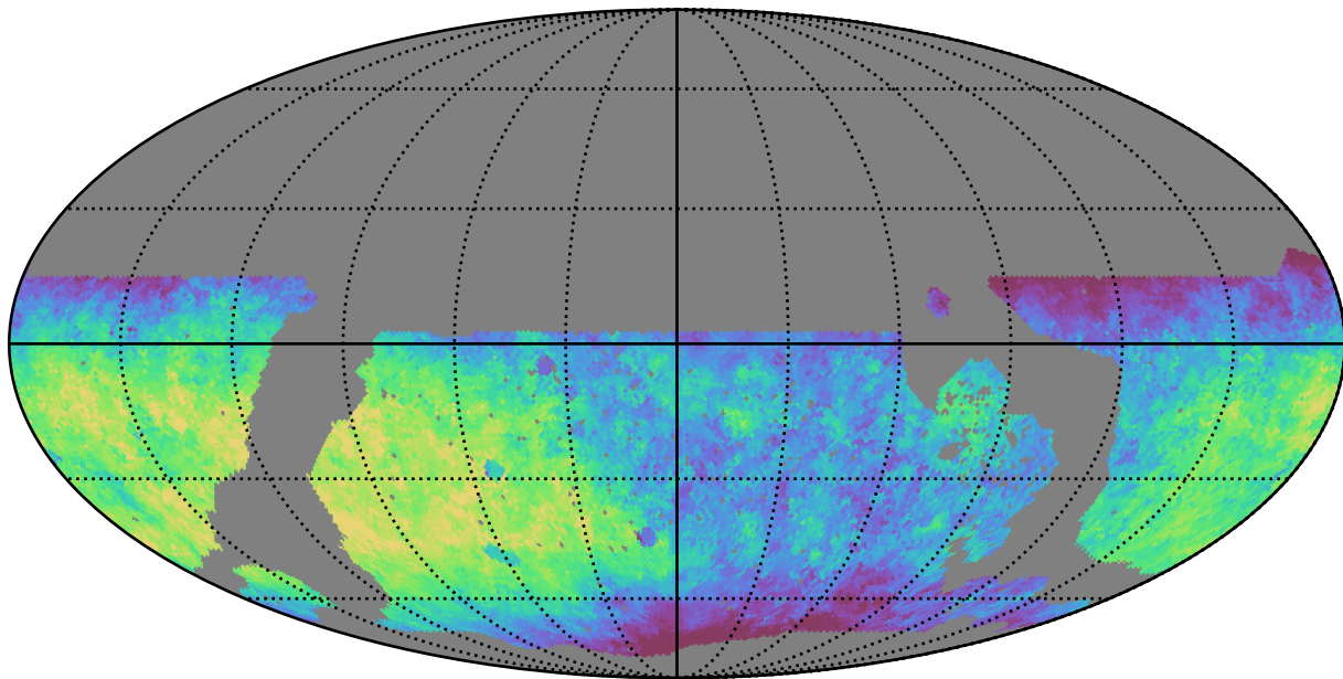
noroll_v3.4_10yrs WFD z band: Median saturation_mag
