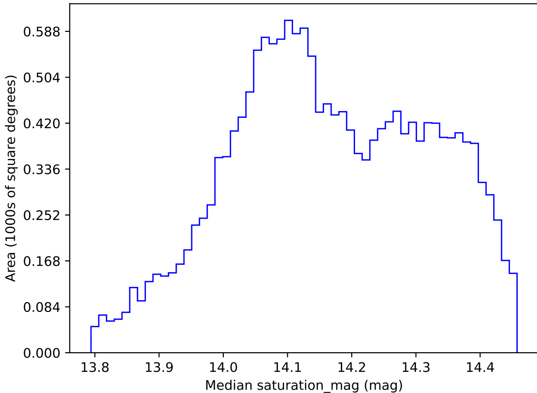
noroll_v3.4_10yrs WFD z band: Median saturation_mag
