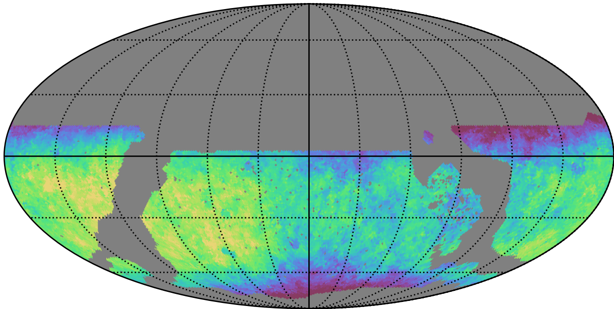
noroll_v3.4_10yrs WFD y band: Median saturation_mag
