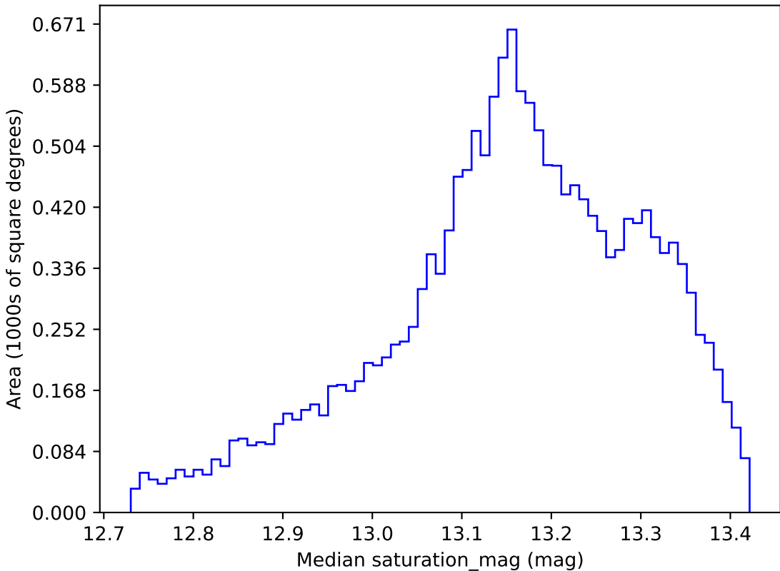
noroll_v3.4_10yrs WFD y band: Median saturation_mag
