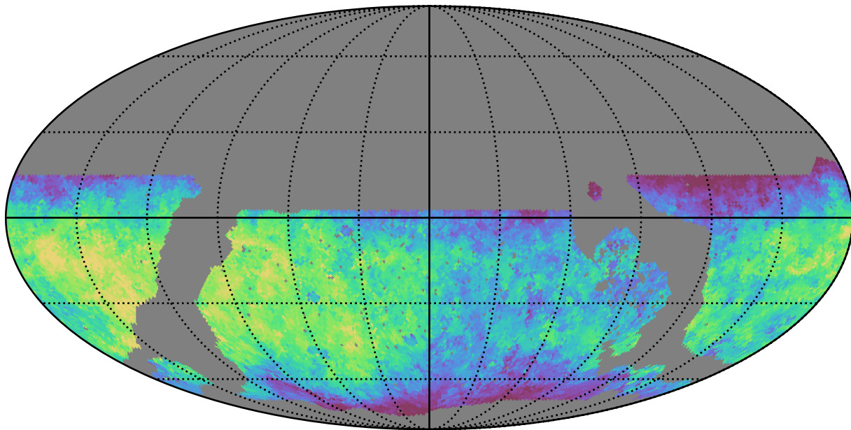
noroll_v3.4_10yrs WFD u band: Median saturation_mag
