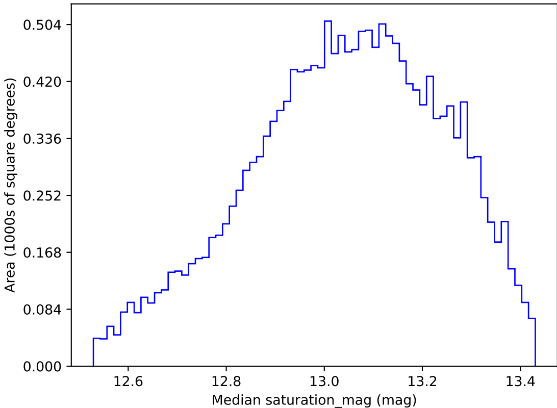
noroll_v3.4_10yrs WFD u band: Median saturation_mag
