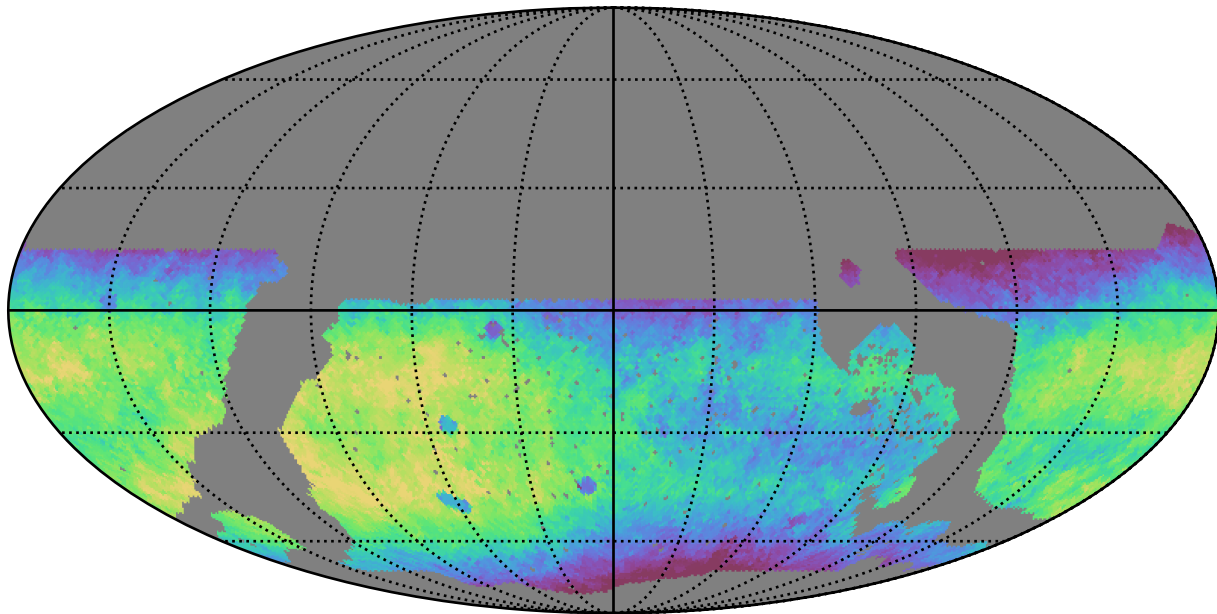
noroll_v3.4_10yrs WFD r band: Median saturation_mag
