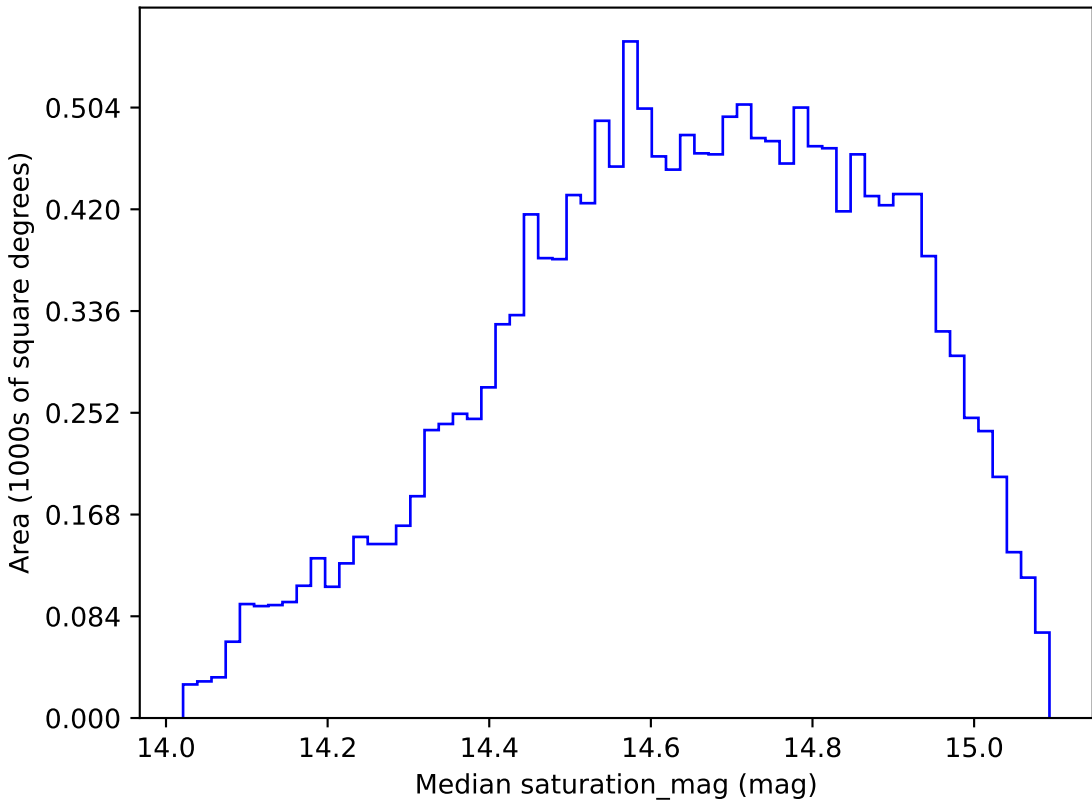
noroll_v3.4_10yrs WFD g band: Median saturation_mag
