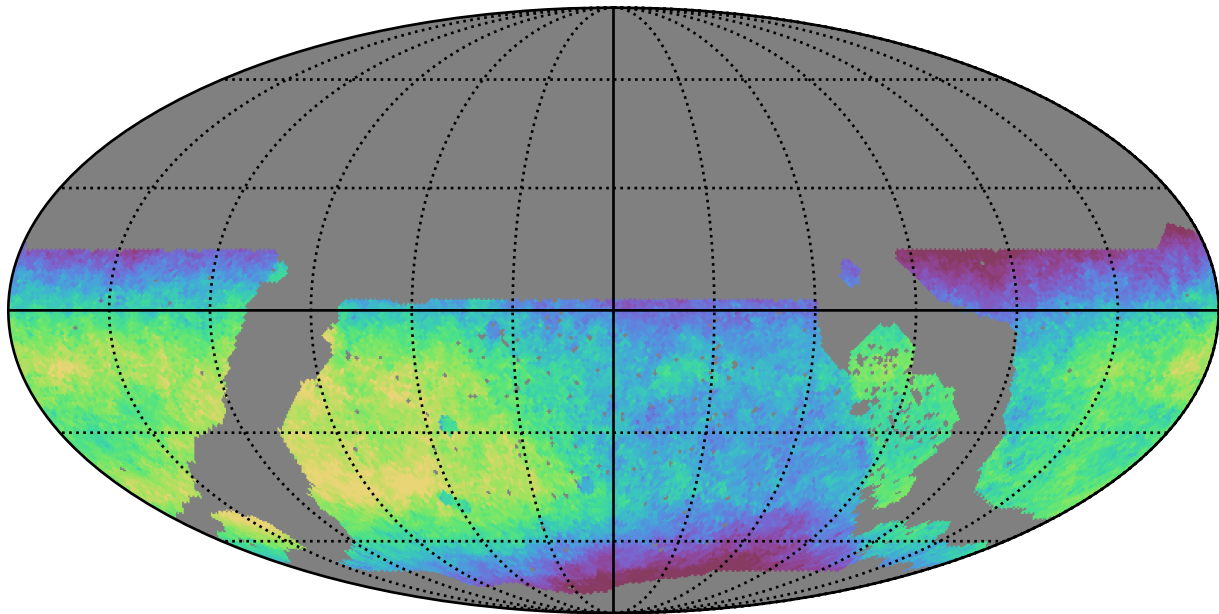
noroll_v3.4_10yrs WFD all bands: Median saturation_mag
