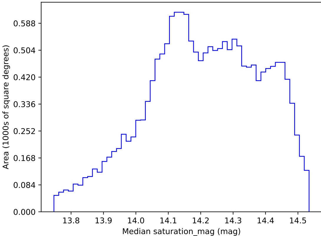
noroll_v3.4_10yrs WFD all bands: Median saturation_mag
