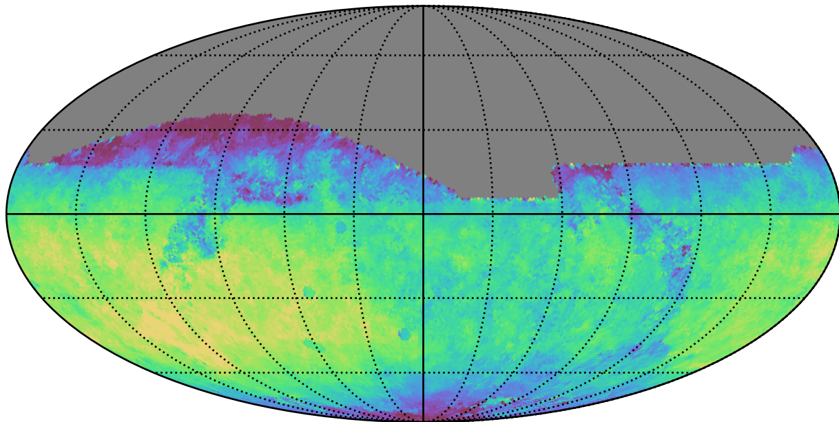
noroll_v3.4_10yrs All sky z band: Median saturation_mag
