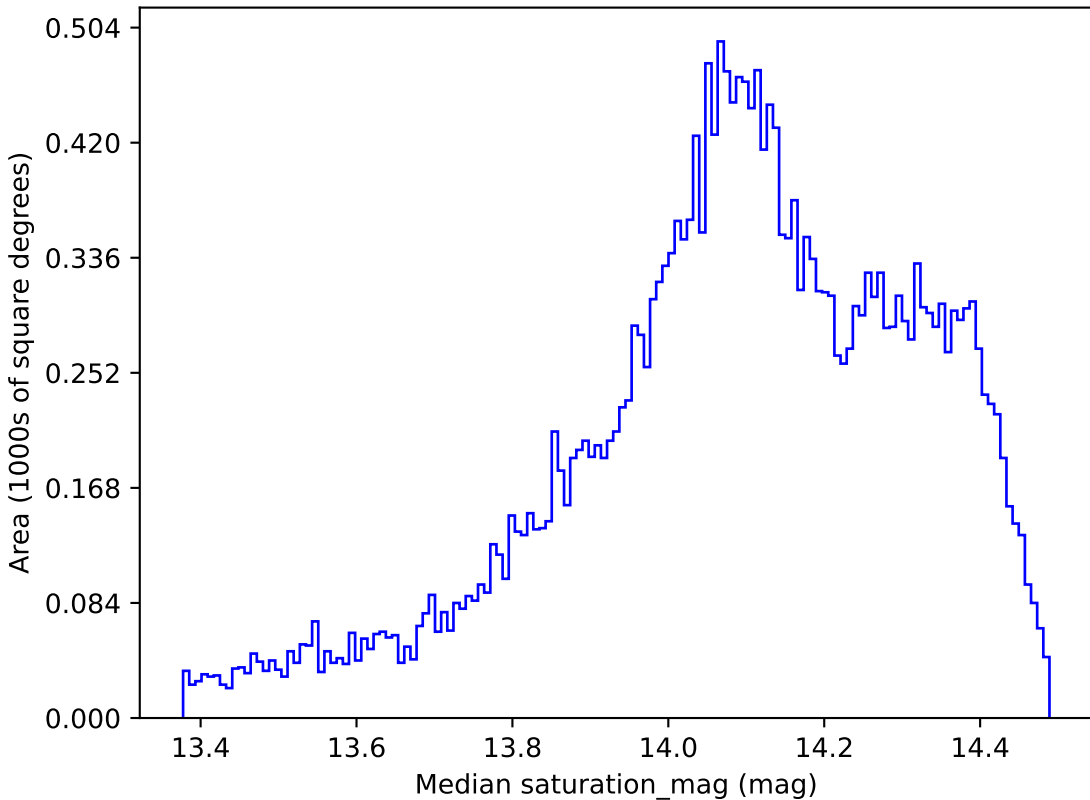
noroll_v3.4_10yrs All sky z band: Median saturation_mag
