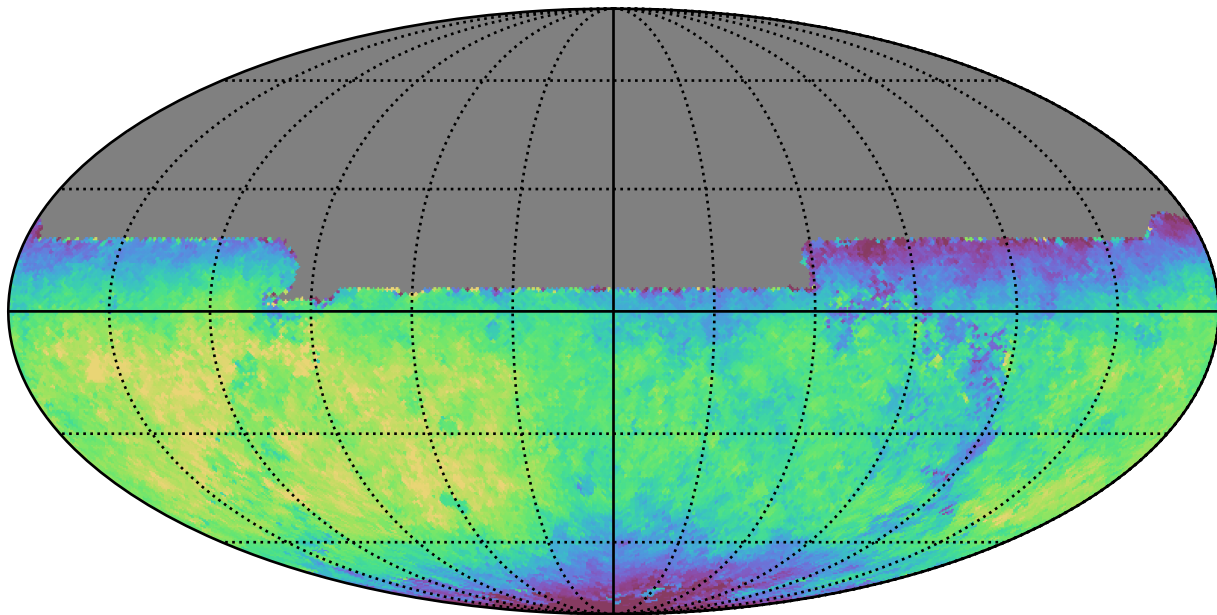
noroll_v3.4_10yrs All sky y band: Median saturation_mag
